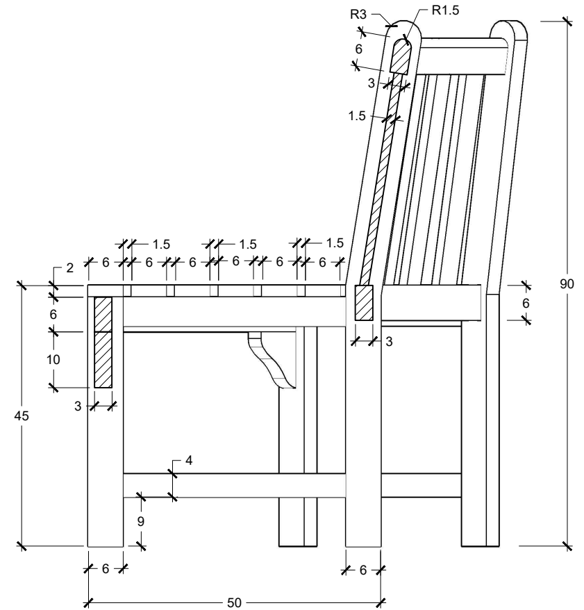
SIDE A-A SCALE 1:9
