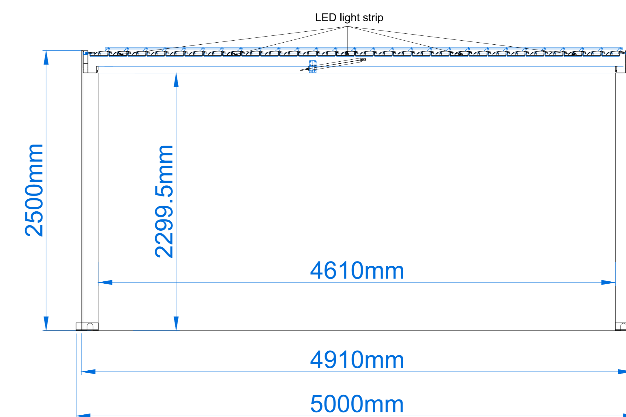
ELEVATION VIEW-2
