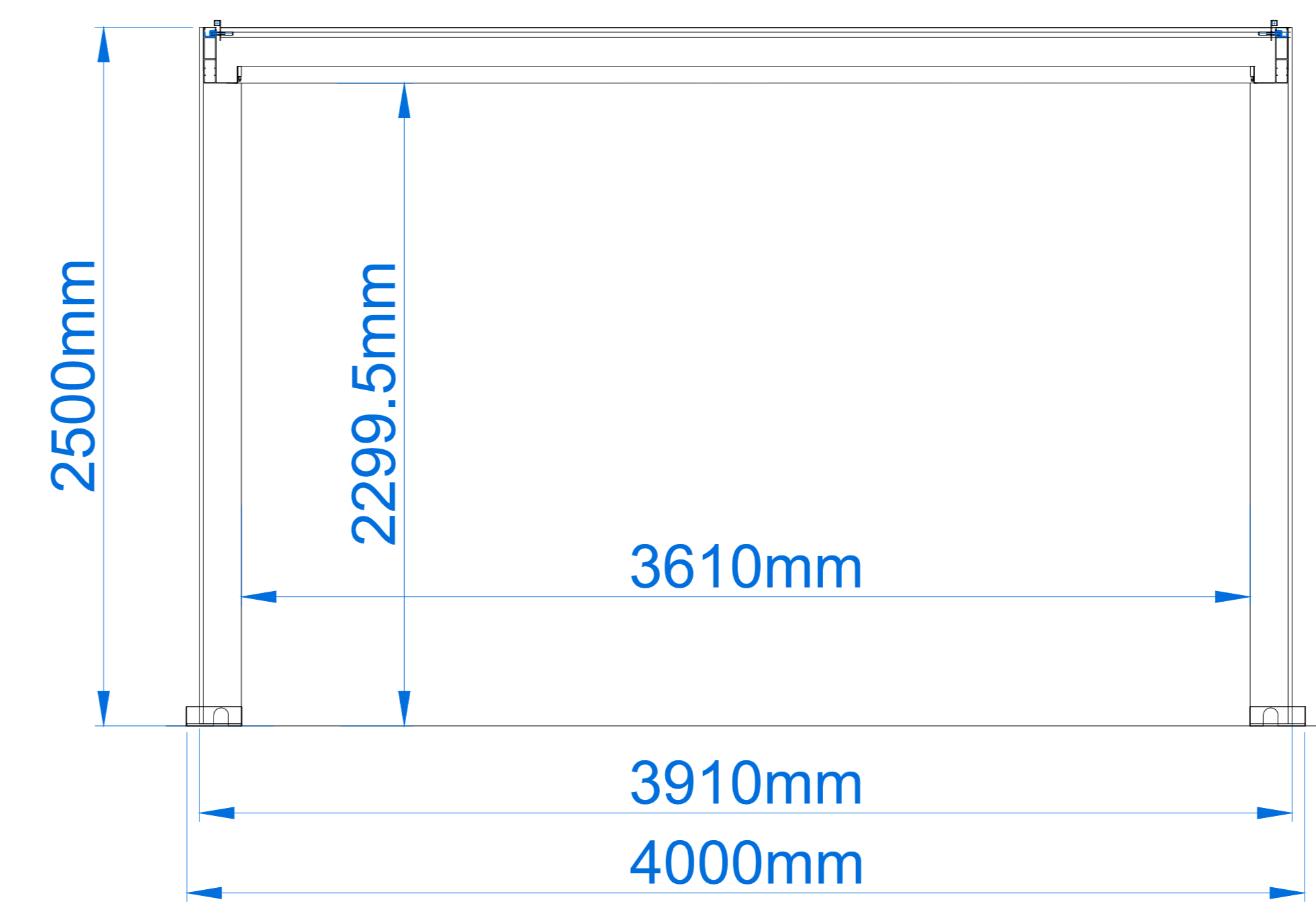
ELEVATION VIEW-1
