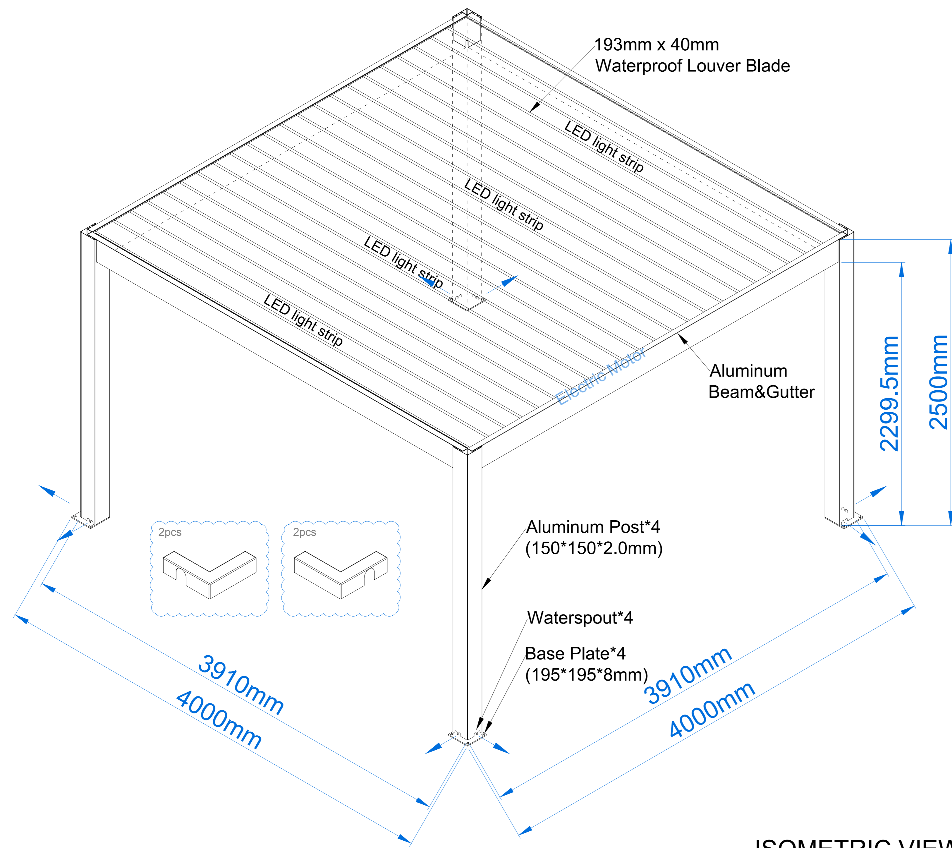
ISOMETRIC VIEW
