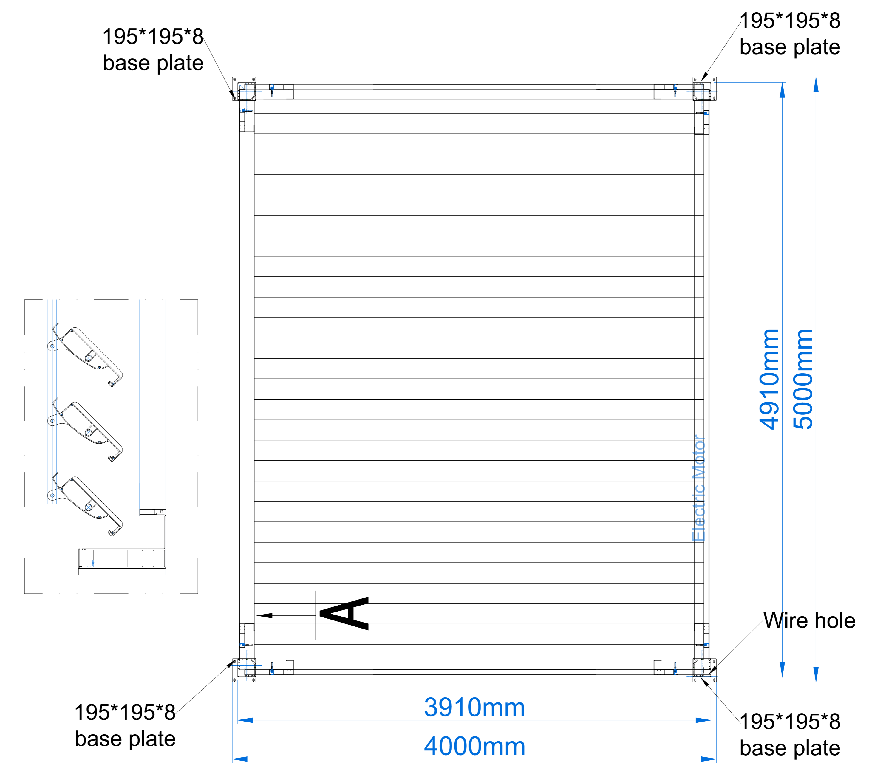
PLAN VIEW
