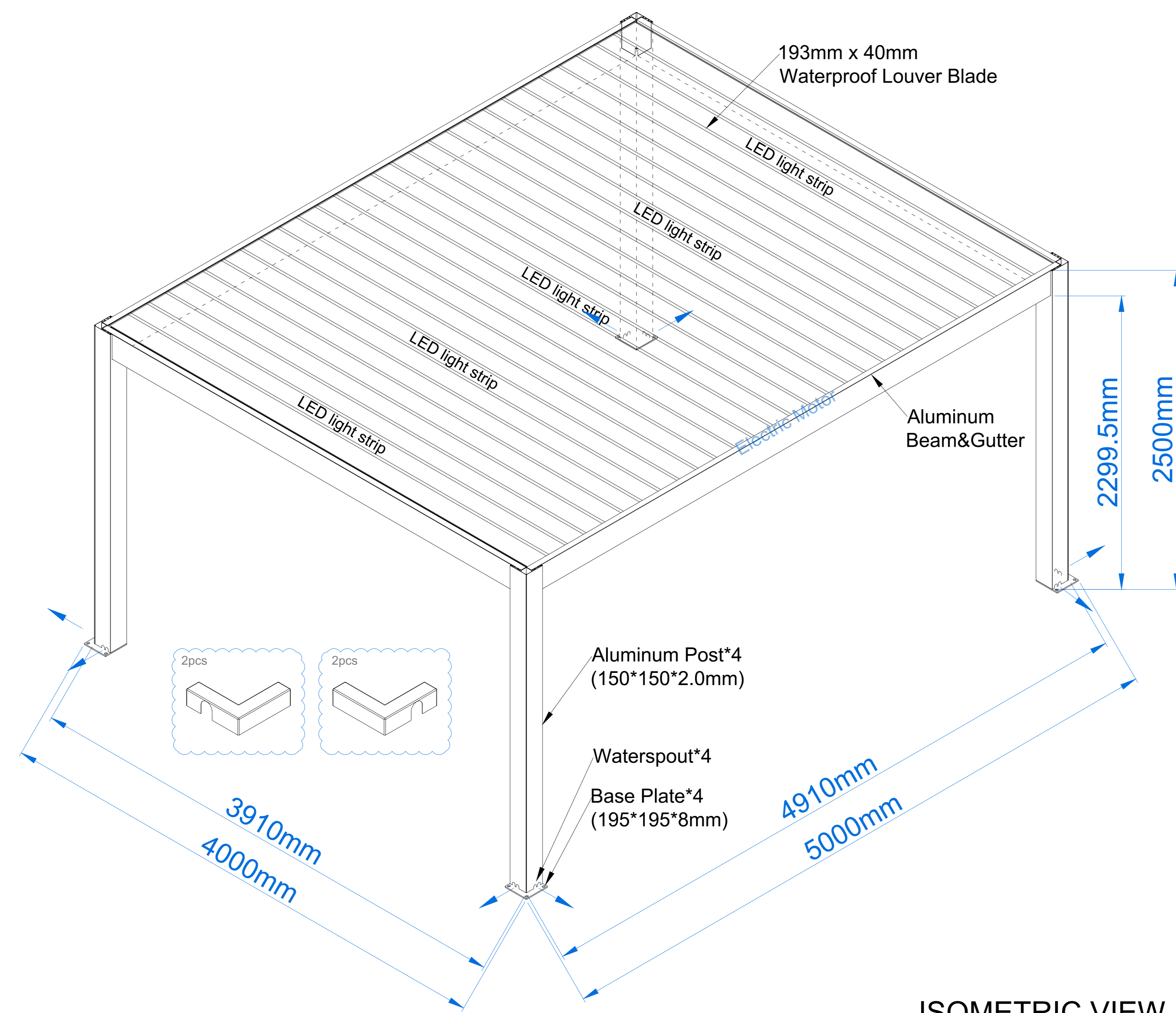
ISOMETRIC VIEW
