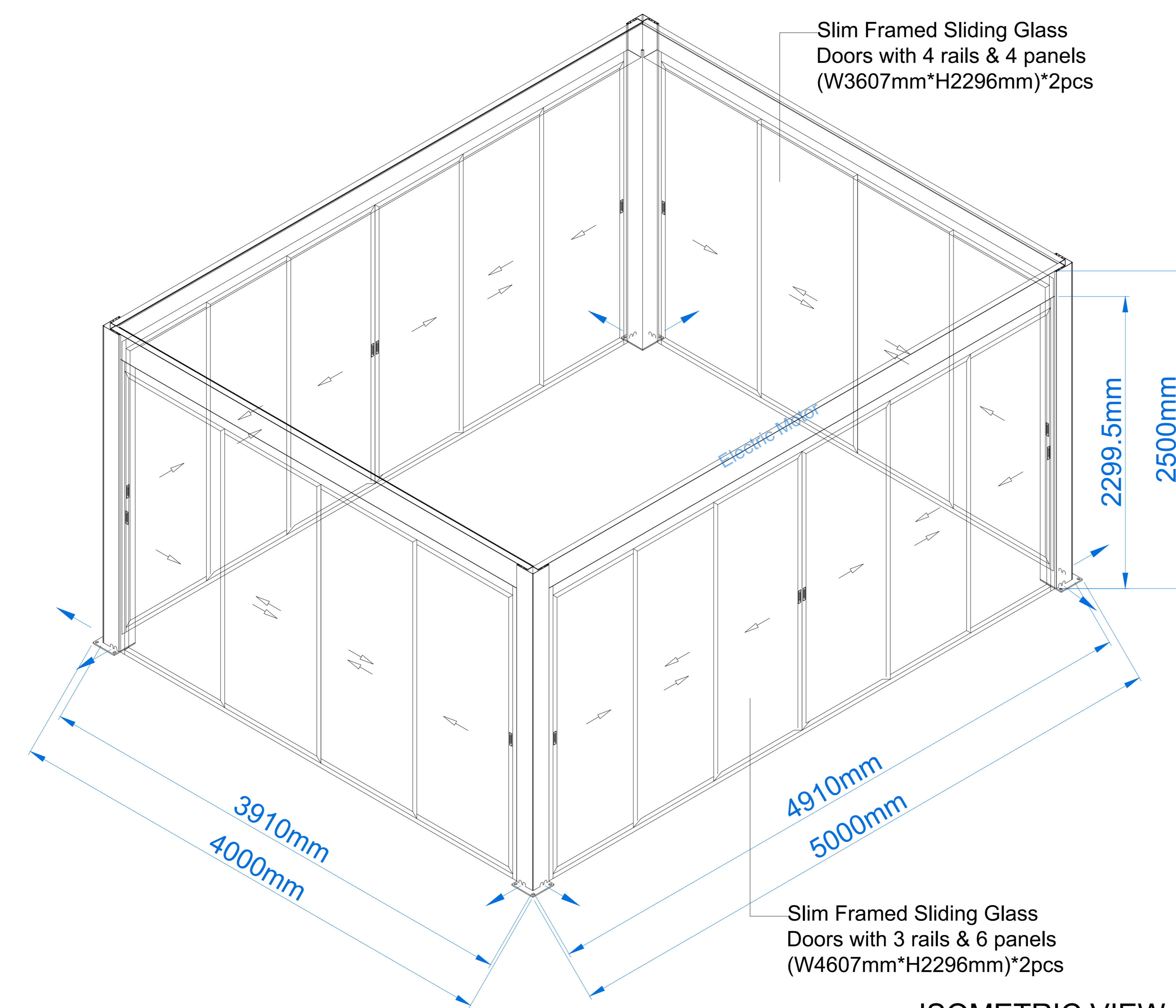
ISOMETRIC VIEW
