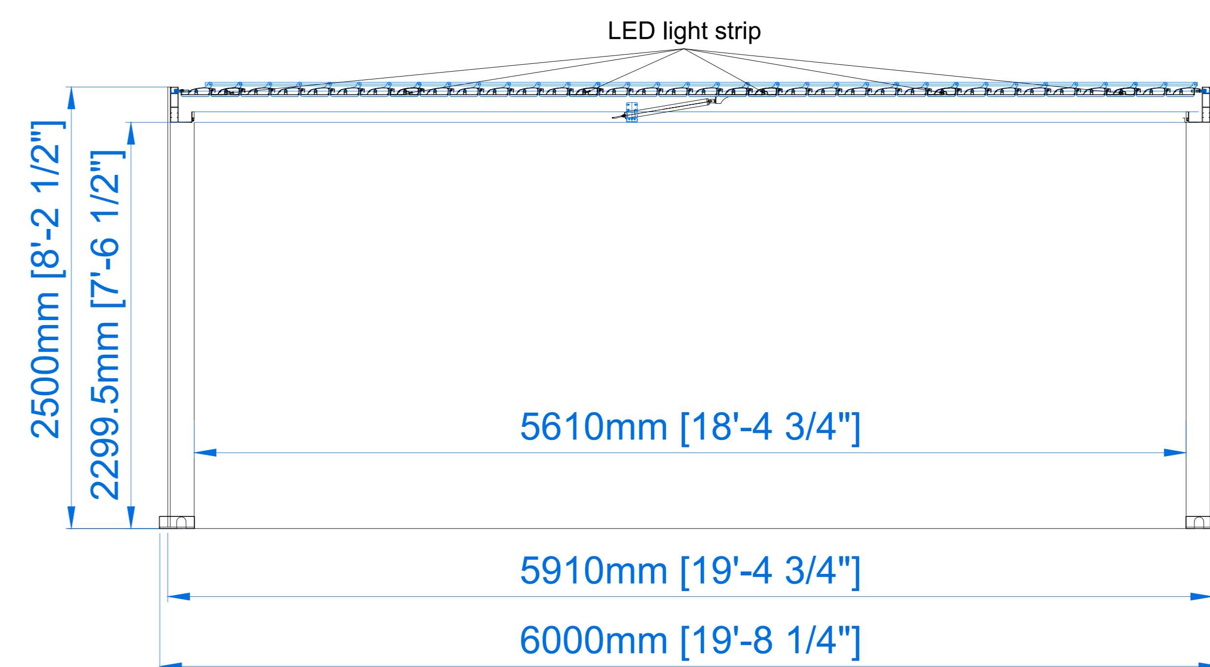
ELEVATION VIEW-2
