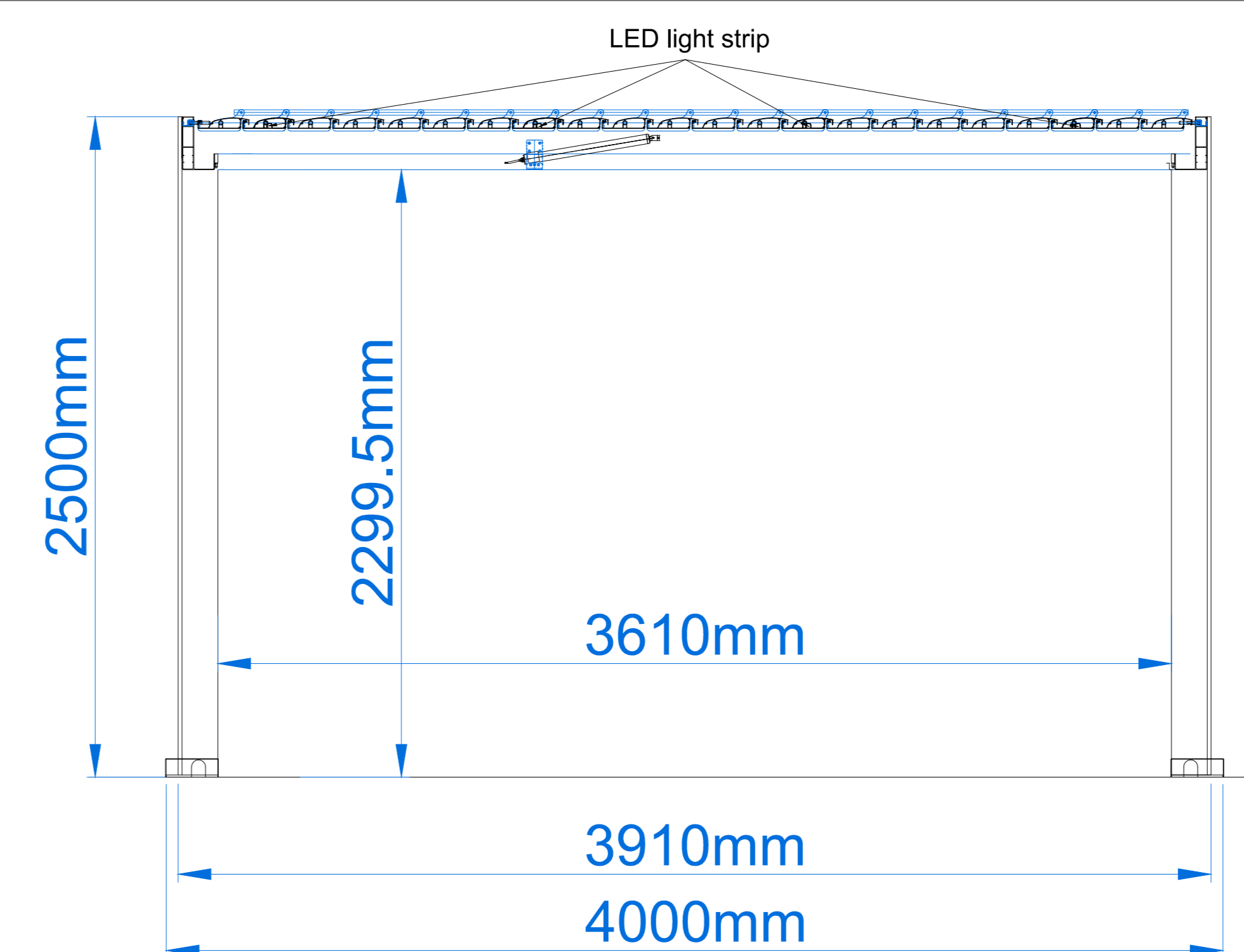
ELEVATION VIEW-2
